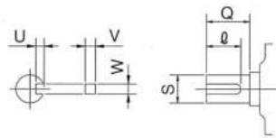
Shaft end
