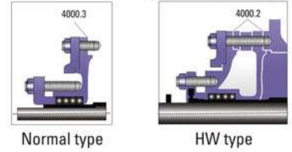
Cross section of stuffing box for MML 40, 50, 65
