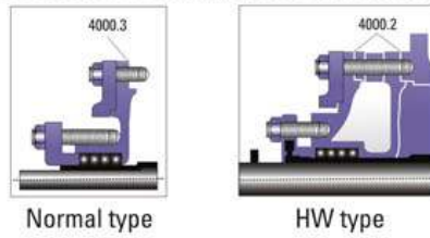
Cross section of stuffing box for MMK 40, 50, 65
